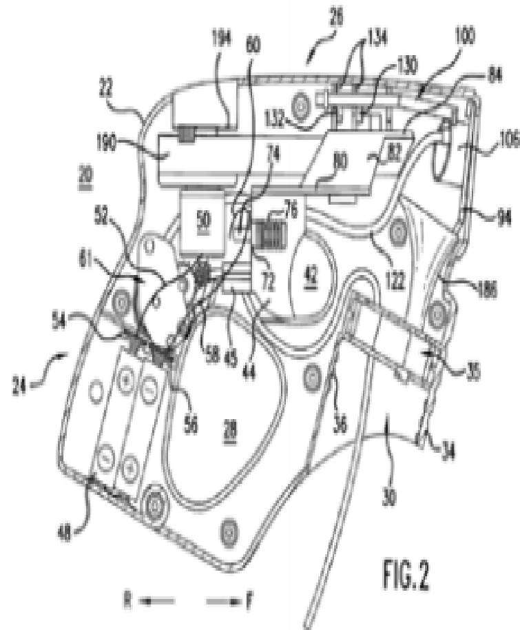
Example of patent application drawing for a "bubble generating assembly" 24
